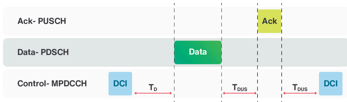
Figure 3.5: Downlink data transfer
