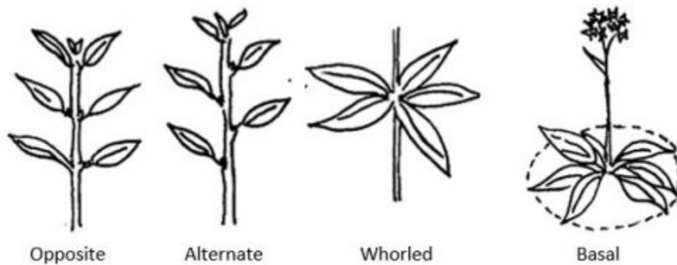
Figure 14.3 Common types of leaf arrangements.
