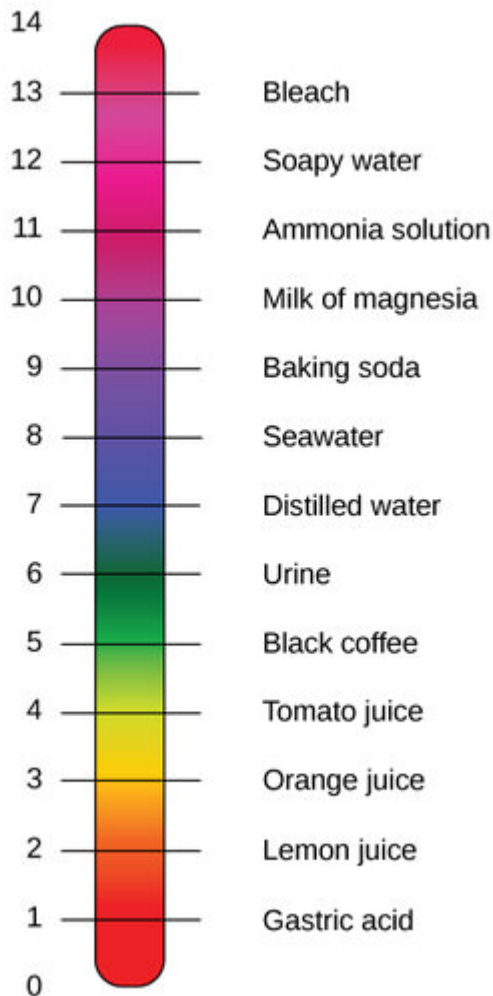
Figure 4. The \text{pH} scale measures the amount of hydrogen ions ( \text{H}^+ ) in a substance. (credit: modification of work by Edward Stevens)
