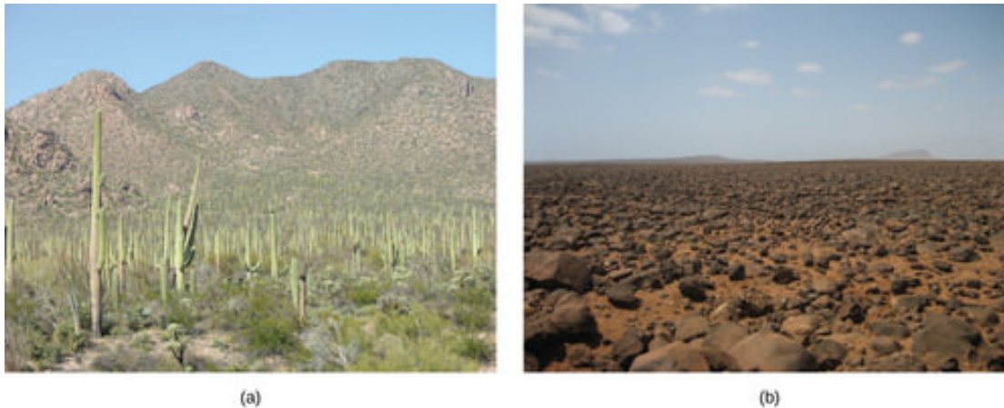
Figure 2. Desert ecosystems, like all ecosystems, can vary greatly. The desert in (a) Saguaro National Park, Arizona, has abundant plant life, while the rocky desert of (b) Boa Vista island, Cape Verde, Africa, is devoid of plant life. (credit a: modification of work by Jay Galvin; credit b: modification of work by Ingo Wölbern)
