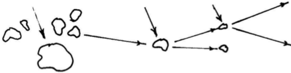
Figure 9. Diastatic activity.
